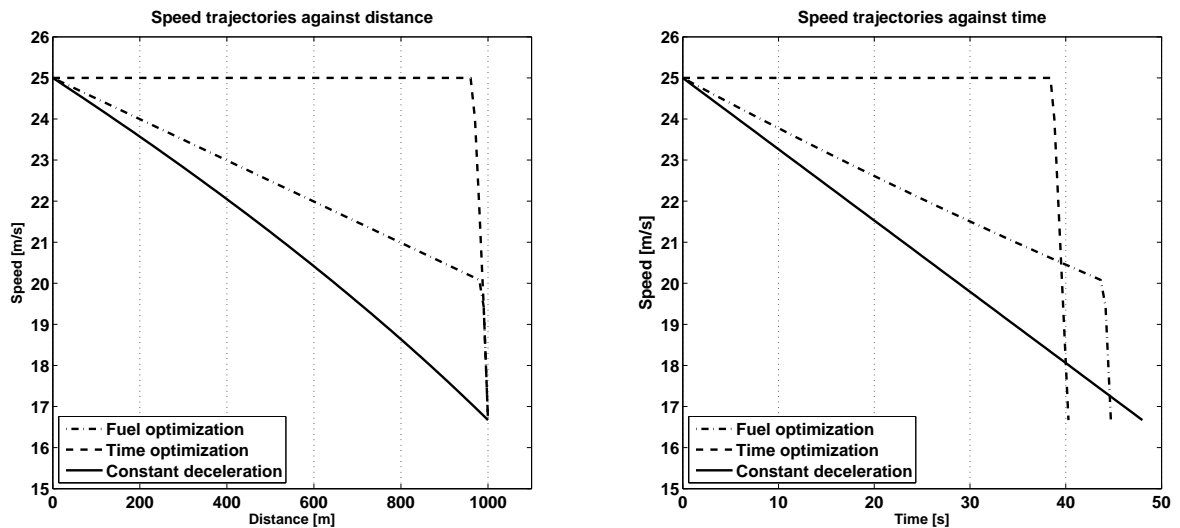
Figure 2. Theoretical speed trajectories for an HDV minimizing fuel consumption, travel time or using constant deceleration from 90 km/h to 60 km/h in 1000 m.
